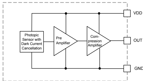
Figure 1 – Simplified block Diagram
